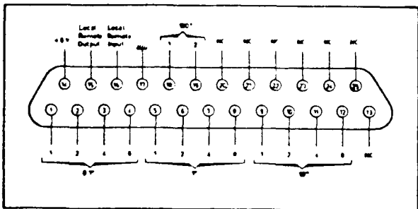
Figure VII-7 CONNECTOR (S012)
